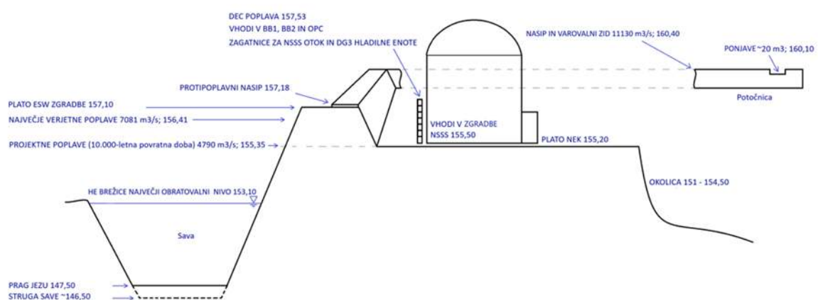
Figure 7: Flood protection
