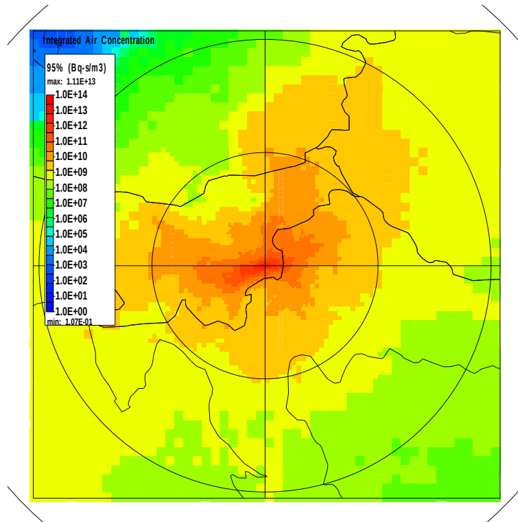
Figure 138: 95th percentile values for integrated concentrations of isotope activity for Xe-133 ( \text{Bq-s/m}^3 ) for design extension conditions, DIPCOT for the year 2020 (source: /196/)
