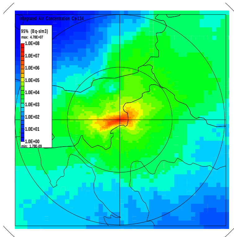
Figure 119: 95th percentile values for integrated concentrations of isotope activity for Cs-134 (Bq-s/m³) for a design basis accident, DIPCOT for the year 2020 (source: /196/)
