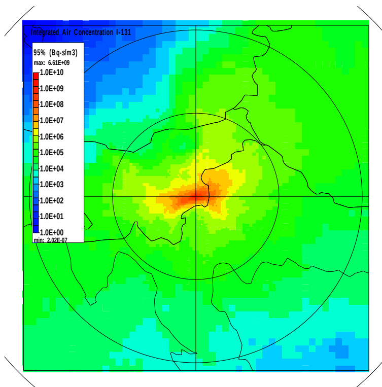
Figure 136: 95th percentile values for integrated concentrations of isotope activity for I-131 (Bq-s/m³) for design extension conditions, DIPCOT for the year 2020 (source: /196/)
