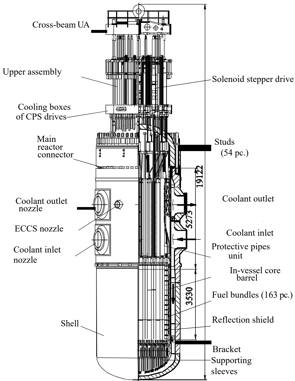
Fig. 3 – Reactor
